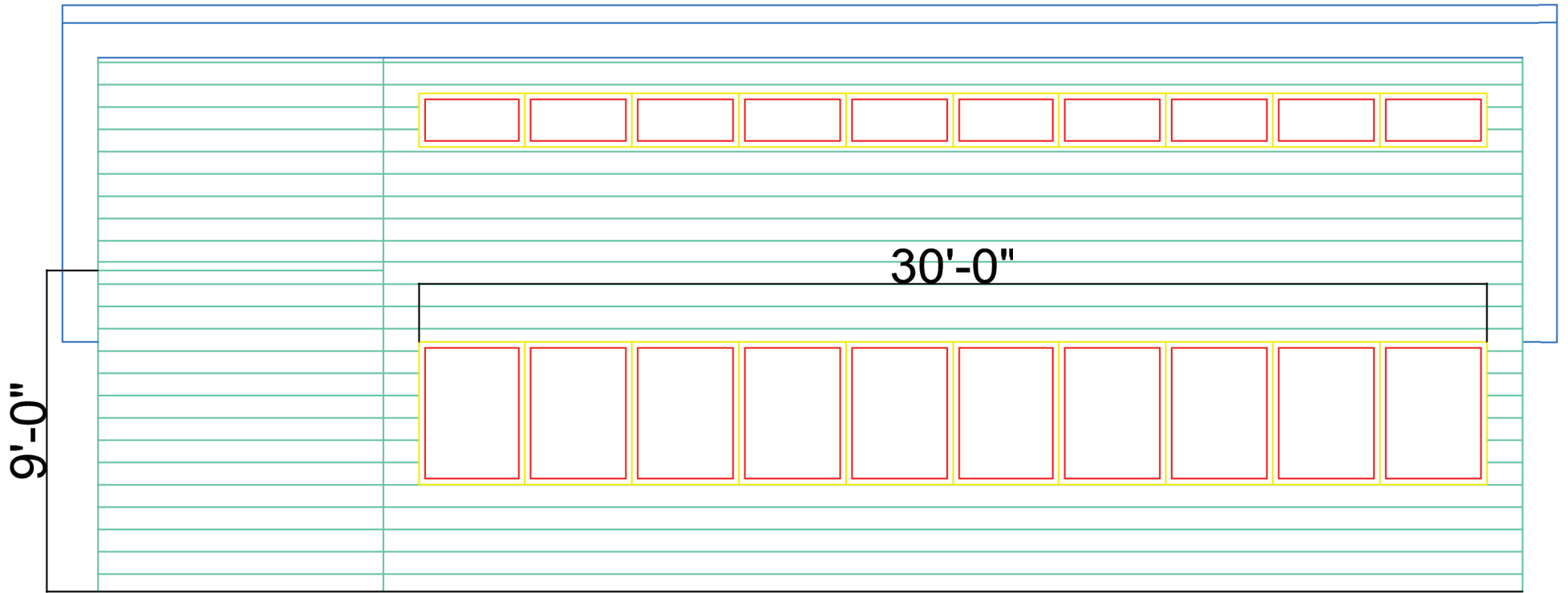
EAST ELEVATION
