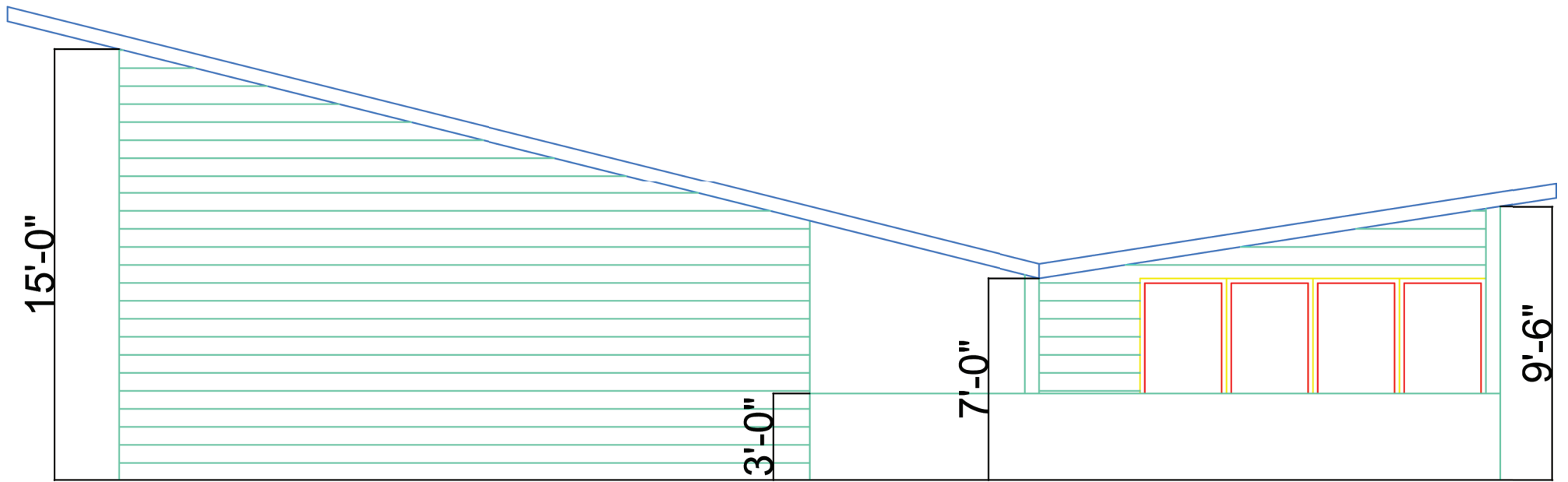
NORTH ELEVATION
