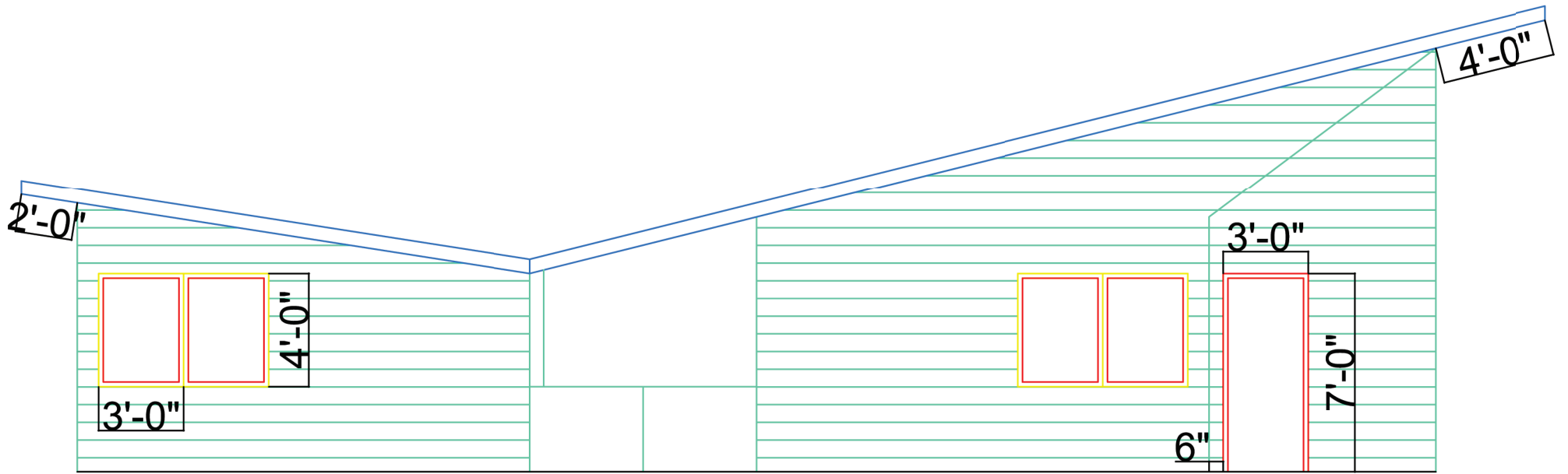
SOUTH ELEVATION
