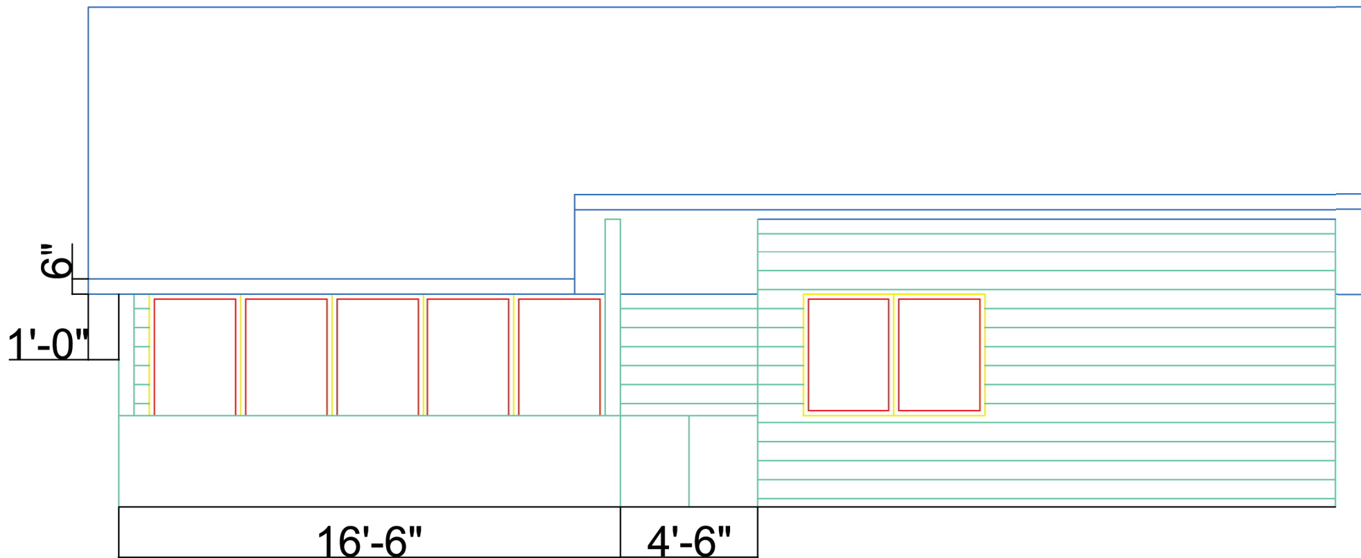
WEST ELEVATION
